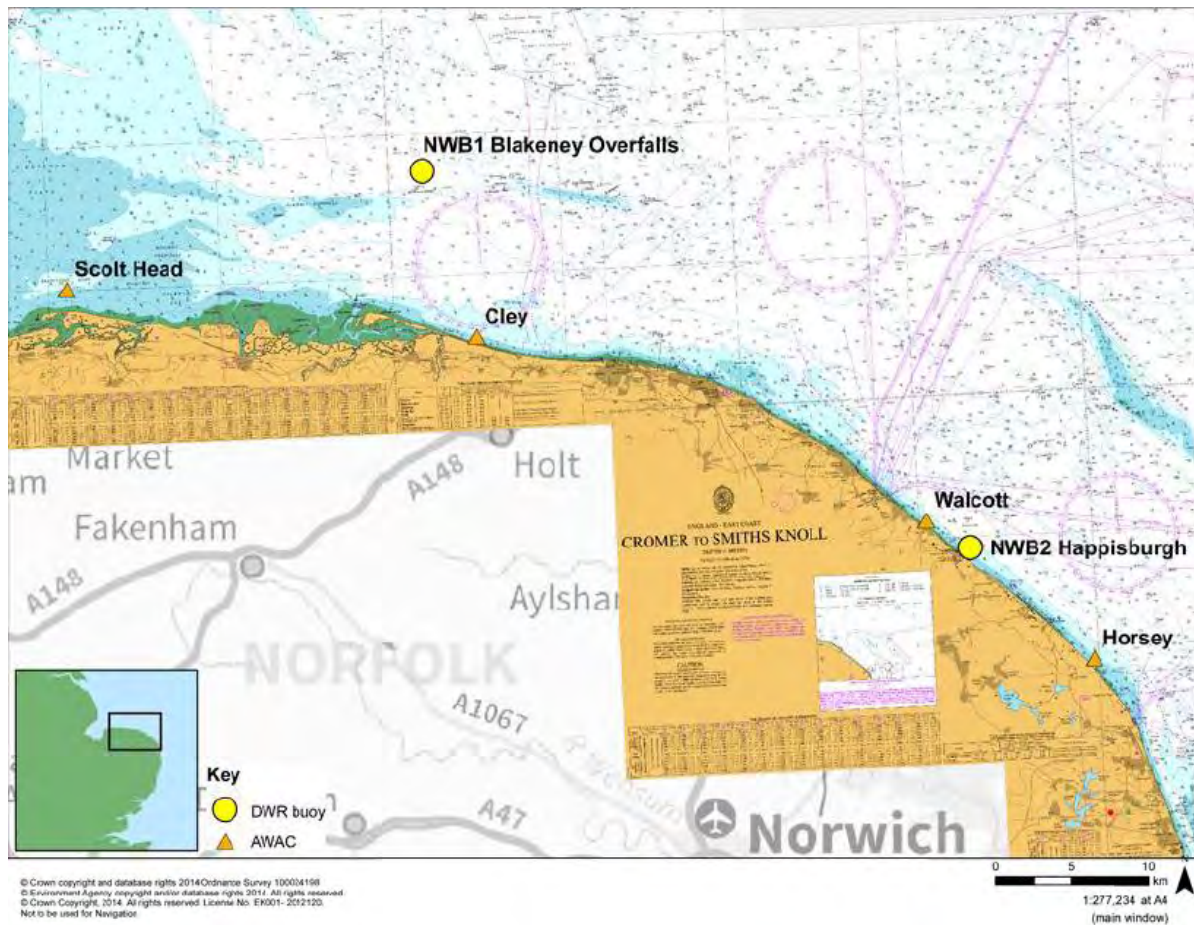
Figure 19 Environment Agency Met Instrument Locations in Norfolk (EA)
